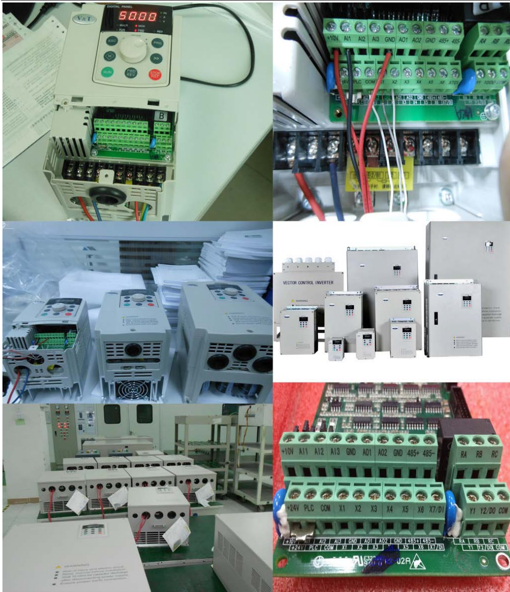
Terminals of our V5 series AC inverter drives (variable speed drives, VSD, VFD)
